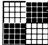
134 &H86 &X10000110
