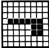
173 &HAD &X10101101
