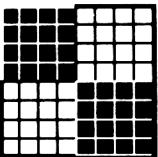
137 &H89 &X10001001
