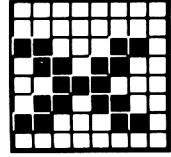
120 &H78 &X01111000
