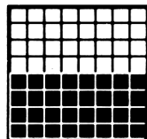
140 &H8C &X10001100
