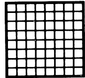
128 &H80 &X10000000
