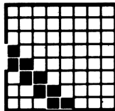
195 &HC3 &X11000011
