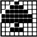
229 &HE5 &X11100101
