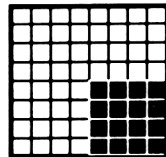
136 &H88 &X10001000
