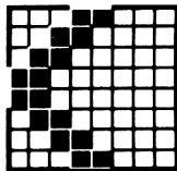
199 &HC7 &X11000111
