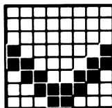
198 &HC6 &X11000110
