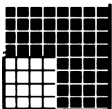
139 &H8B &X10001011
