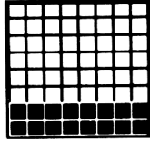
210 &HD2 &X11010010
