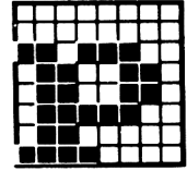
112 &H70 &X01110000
