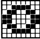
230 &HE6 &X11100110
