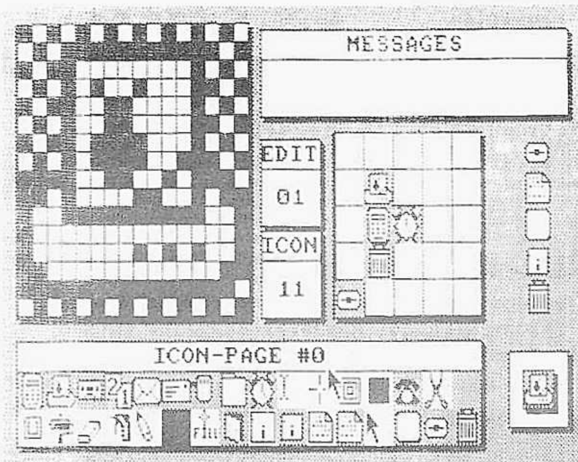
Figure 9 – L'écran Icon Designer
